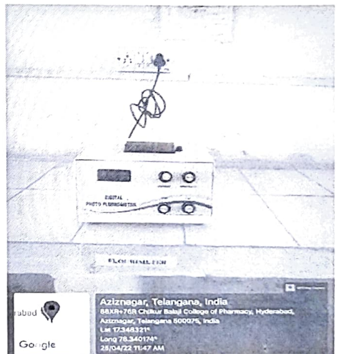
DIGITAL PHOTOFLUOROMETER
