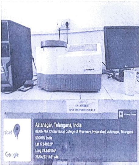
UV-VISIBLE SPECTROPHOTOMETER
