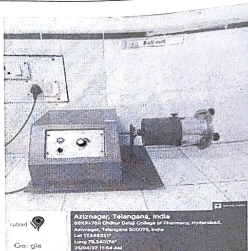
BALL MILL
